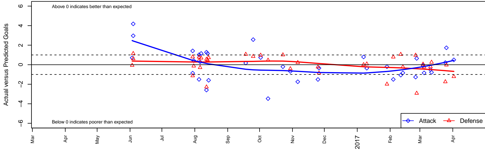
Crossfire Premier A G02 Dots are actual minus expected GF (blue circles) and GA (red triangles). Blue line is smoothed change in attack strength. Red is smoothed change in defense strength.
